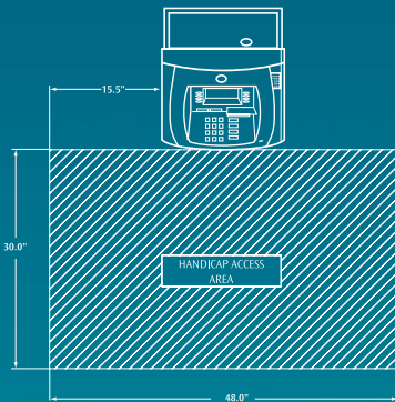
ATM INSTALLATION SPACE REQUIREMENTS FOR ADA COMPLIANCE
